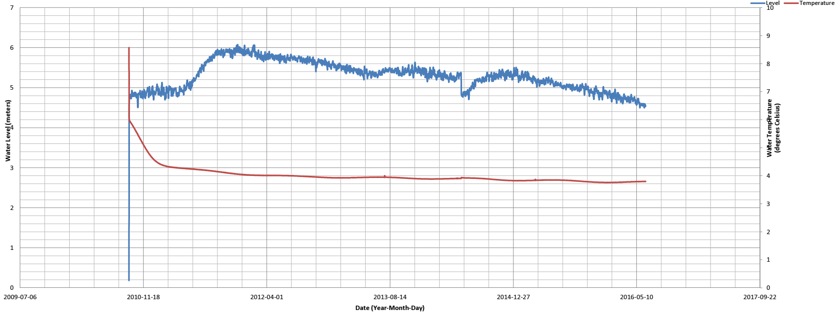
Whitehead/Elton Well Monitoring Readings (South of PTH 1)
